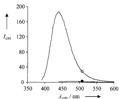
Figure 3. Emission spectra from a monolayer of adsorbate 5 after excitation at \lambda_{\text{ex}} = 350 nm ( \circ ) and \lambda_{\text{ex}} = 420 nm ( \bullet ); I_{\text{cm}} in 10^3 counts \text{s}^{-1} .
